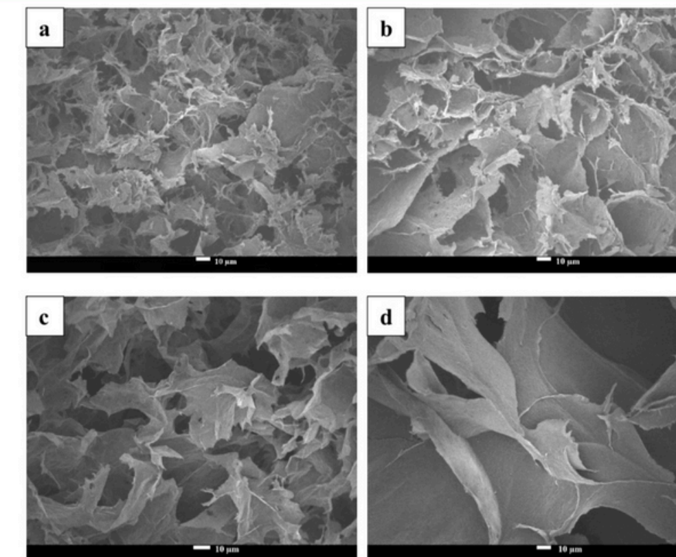
Figure 4. Field emission gun SEM (FEG-SEM) images of a three-dimensional graphene aerogel (scale bar: 10 \mu m): (a) Without ammonia (500 \times ), (b) 0.025% w/v NH 3 (500 \times ), (c) 0.05% w/v NH 3 (600 \times ), and (d) 0.075% w/v NH 3 (500 \times ).
